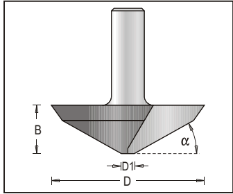
Raised Panel Bit, French Provincial, Plunge Type, 2 Flutes
