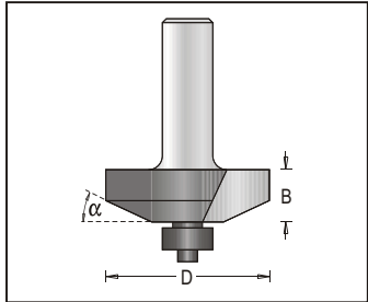
Raised Panel Bit with Ball Bearing Guide, 2 Flutes
