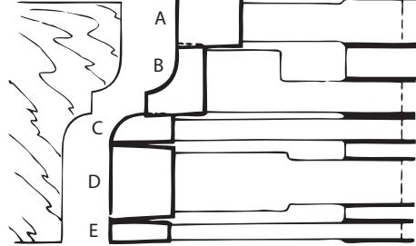
5 Cutter - 1 Pass
