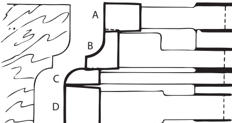
4 Cutter - 1 Pass
