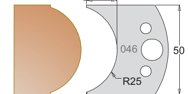
Knife 3304650 Limiter 3404650
