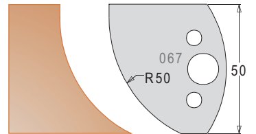
Knife 3306750 Limiter 3406750
