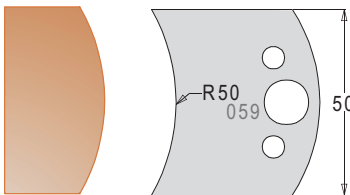
Knife 3305950 Limiter 3405950
