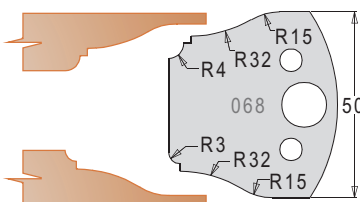
Knife 3306850 Limiter 3406850
