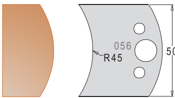
Knife 3305650 Limiter 3405650
