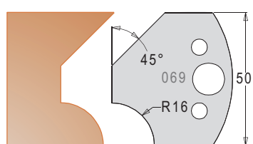
Knife 3306950 Limiter 3406950
