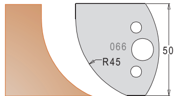
Knife 3306650 Limiter 3406650
