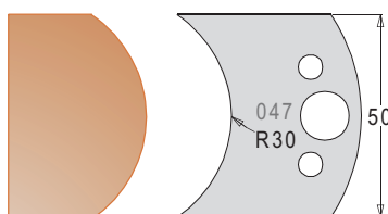
Knife 3304750 Limiter 3404750
