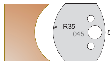
Knife 3304550 Limiter 3404550
