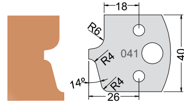
Knife 3304140 Limiter 3404140
