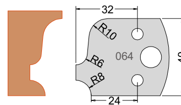
Knife 3306440 Limiter 3406440
