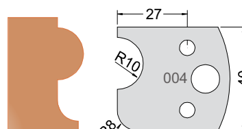
Knife 3300440 Limiter 3400440
