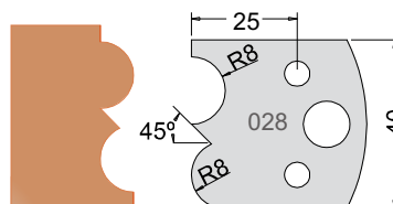
Knife 3302840 Limiter 3402840
