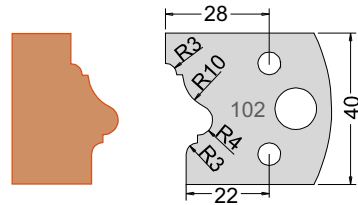
Knife 3310240 Limiter 3410240
