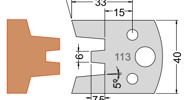
Knife 3311340 Limiter 3411340
