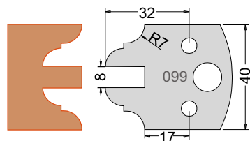
Knife 3309940 Limiter 3409940
