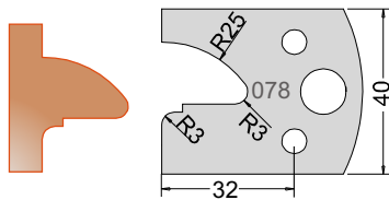
Knife 3307840 Limiter 3407840
