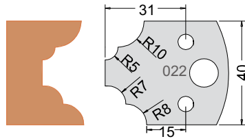
Knife 3302240 Limiter 3402240
