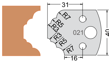
Knife 3302140 Limiter 3402140
