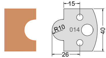
Knife 3301440 Limiter 3401440
