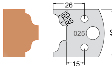
Knife 3302540 Limiter 3402540
