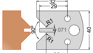
Knife 3307140 Limiter 3407140
