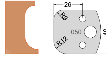
Knife 3305040 Limiter 3405040
