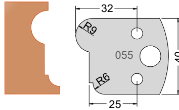
Knife 3305540 Limiter 3405540
