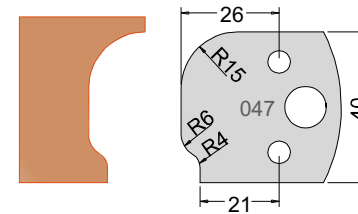
Knife 3304740 Limiter 3404740
