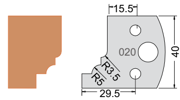
Knife 3302040 Limiter 3402040
