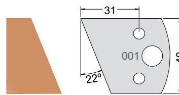
Knife 3300140 Limiter 3400140
