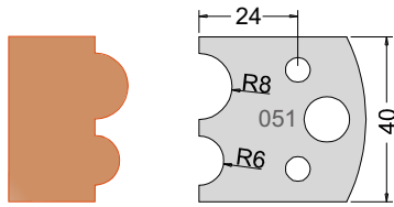
Knife 3305140 Limiter 3405140
