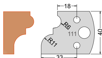
Knife 3311140 Limiter 3411140
