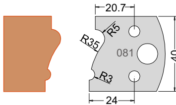
Knife 3308140 Limiter 3408140
