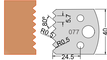
Knife 3307740 Limiter 3407740
