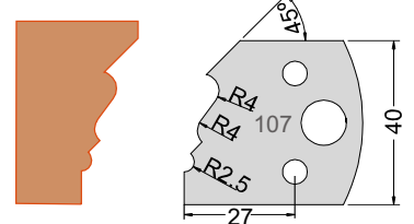
Knife 3310740 Limiter 3410740
