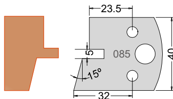
Knife 3308540 Limiter 3408540
