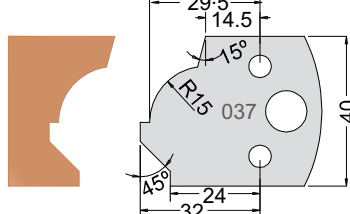
Knife 3303740 Limiter 3403740
