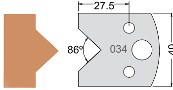
Knife 3303440 Limiter 3403440
