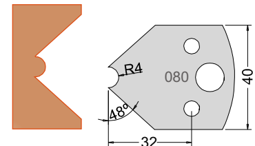
Knife 3308040 Limiter 3408040
