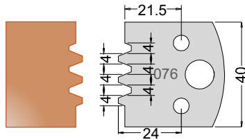
Knife 3307640 Limiter 3407640
