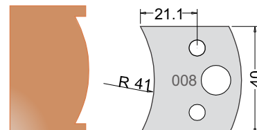
Knife 3300840 Limiter 3400840
