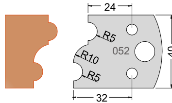
Knife 3305240 Limiter 3405240
