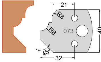
Knife 3307340 Limiter 3407340
