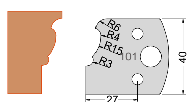
Knife 3310140 Limiter 3410140
