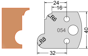
Knife 3305440 Limiter 3405440
