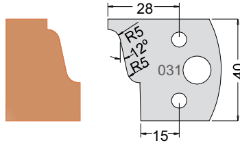
Knife 3303140 Limiter 3403140
