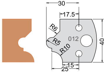
Knife 3301240 Limiter 3401240
