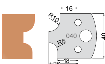
Knife 3304040 Limiter 3404040
