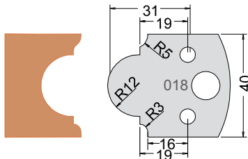
Knife 3301840 Limiter 3401840
