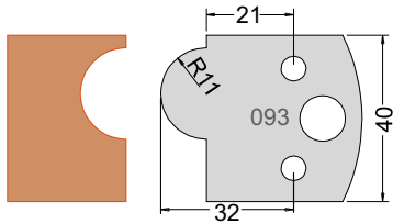
Knife 3309340 Limiter 3409340
