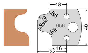
Knife 3305640 Limiter 3405640
