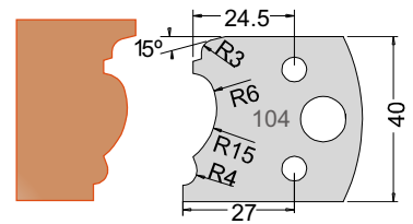
Knife 3310440 Limiter 3410440
