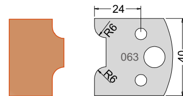
Knife 3306340 Limiter 3406340
