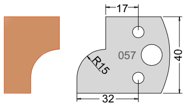
Knife 3305740 Limiter 3405740
