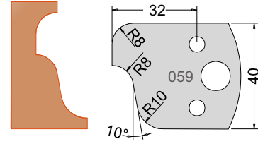
Knife 3305940 Limiter 3405940
