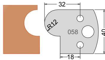
Knife 3305840 Limiter 3405840
