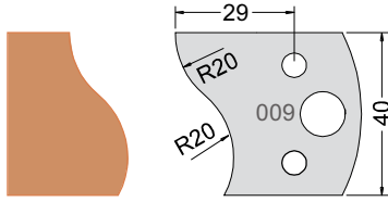
Knife 3300940 Limiter 3400940
