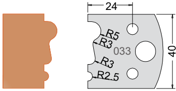
Knife 3303340 Limiter 3403340
