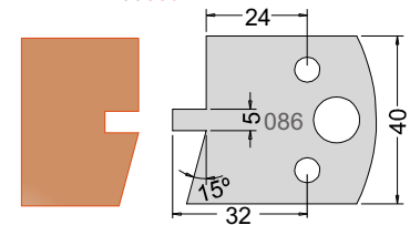
Knife 3308640 Limiter 3408640
