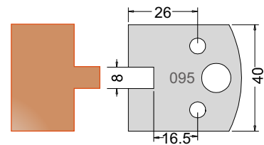
Knife 3309540 Limiter 3409540
