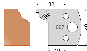
Knife 3306740 Limiter 3406740
