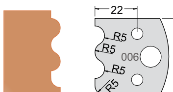
Knife 3300640 Limiter 3400640
