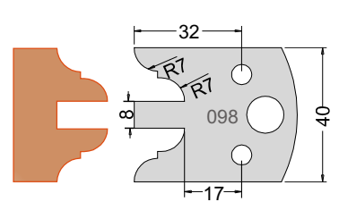
Knife 3309840 Limiter 3409840
