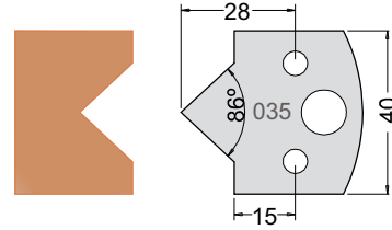
Knife 3303540 Limiter 3403540
