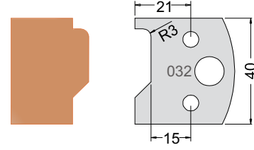
Knife 3303240 Limiter 3403240
