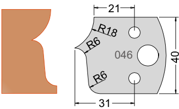
Knife 3304640 Limiter 3404640
