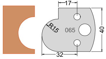
Knife 3306540 Limiter 3406540
