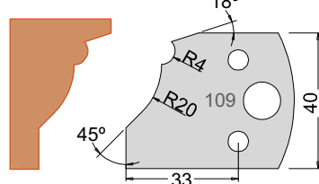
Knife 3310940 Limiter 3410940
