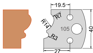
Knife 3310540 Limiter 3410540
