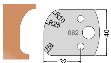
Knife 3306240 Limiter 3406240
