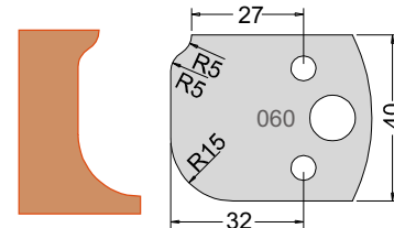
Knife 3306040 Limiter 3406040
