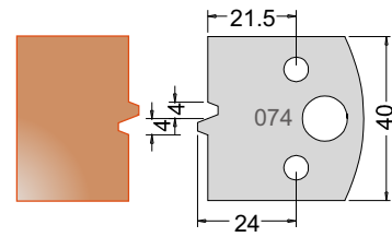
Knife 3307440 Limiter 3407440
