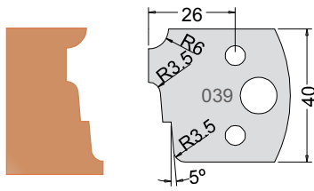
Knife 3303940 Limiter 3403940
