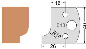
Knife 3301340 Limiter 3401340
