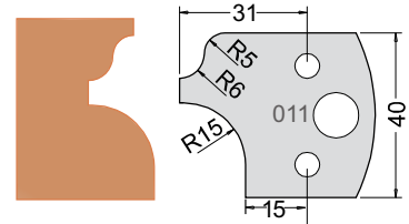
Knife 3301140 Limiter 3401140
