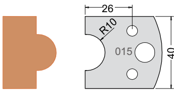
Knife 3301540 Limiter 3401540
