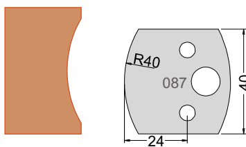
Knife 3308740 Limiter 3408740
