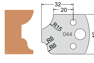
Knife 3304440 Limiter 3404440
