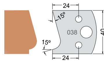
Knife 3303840 Limiter 3403840
