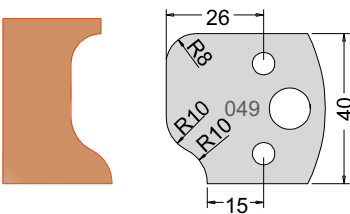
Knife 3304940 Limiter 3404940
