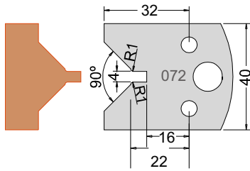
Knife 3307240 Limiter 3407240
