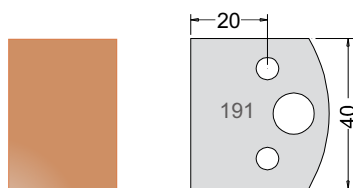
Knife 3319140 Limiter 3419140
