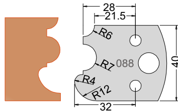
Knife 3308840 Limiter 3408840
