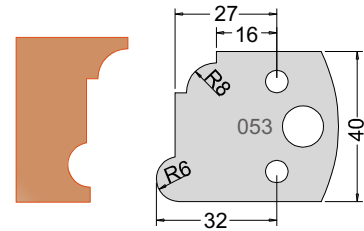
Knife 3305340 Limiter 3405440
