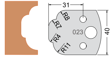
Knife 3302340 Limiter 3402340
