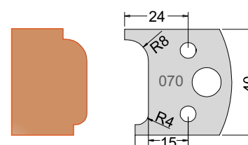
Knife 3307040 Limiter 3407040
