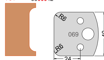
Knife 3306940 Limiter 3406940
