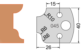
Knife 3304540 Limiter 3404540
