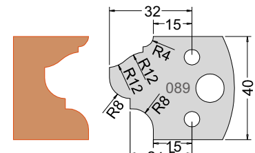
Knife 3308940 Limiter 3408940
