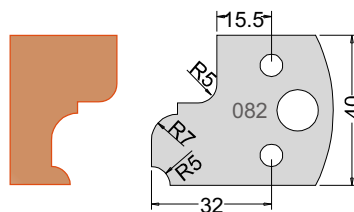
Knife 3308240 Limiter 3408240
