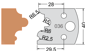
Knife 3303640 Limiter 3403640
