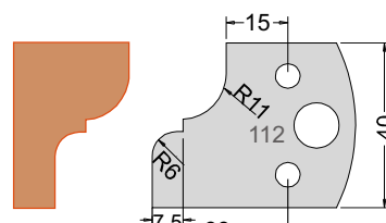
Knife 3311240 Limiter 3411240
