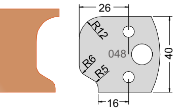
Knife 3304840 Limiter 3404840
