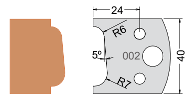
Knife 3300240 Limiter 3400240
