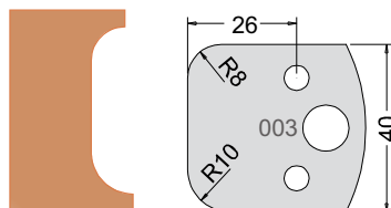
Knife 3300340 Limiter 3400340
