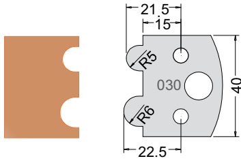
Knife 3303040 Limiter 3403040
