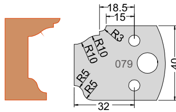
Knife 3307940 Limiter 3407940
