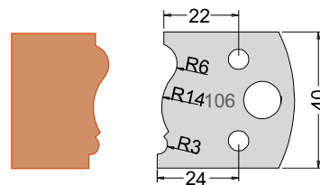
Knife 3310640 Limiter 3410640
