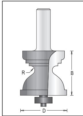
Moulding Bit, 2 Flutes
