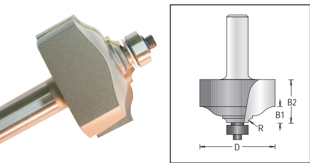
Edge Forming Bits, 2 Flutes
