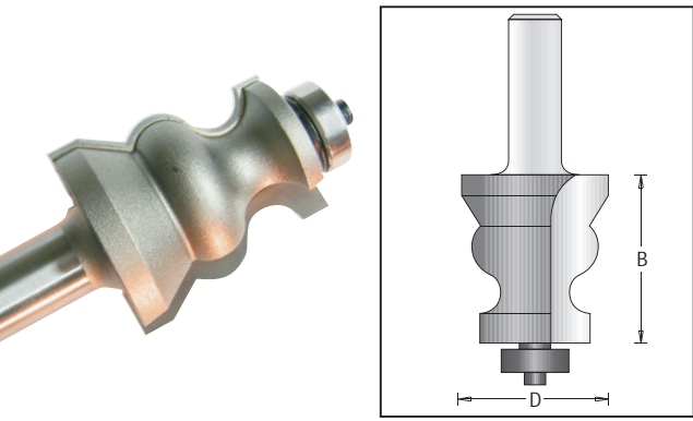
Edge Forming Bits, 2 Flutes
