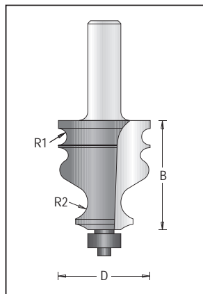
Edge Forming Bit, 2 Flutes
