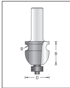
Edge Forming Bit, 2 Flutes
