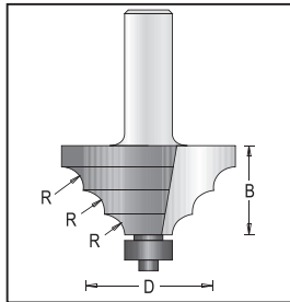
Moulding Bit, 2 Flutes
