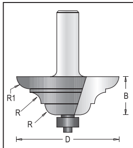
Moulding Bit, 2 Flutes
