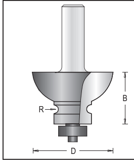
Moulding Bit, 2 Flutes
