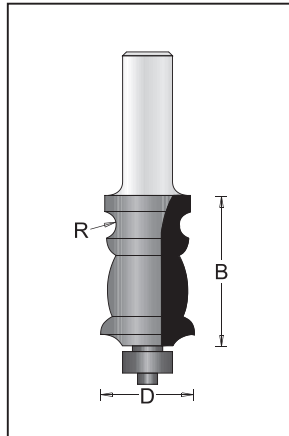
Fancy Moulding Bits, 1/2" Shank, 2 Flutes
