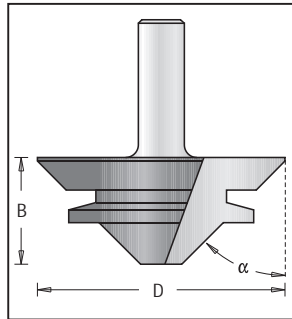
Miter Lock Bits, 2 Flutes
