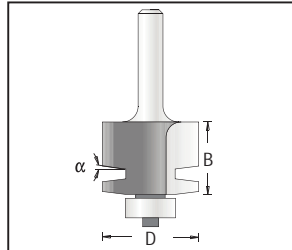
Glue Joint Bit, 2 Flutes
