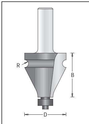
Handrail Bit, 2 Flutes
