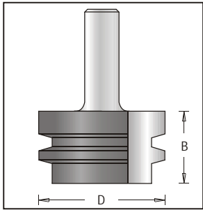
Glue Joint Bit, 2 Flutes
