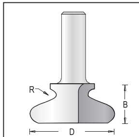
Finger Grip Router Bits, 2 Flutes
