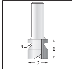
Finger Grip Router Bits, 2 Flutes
