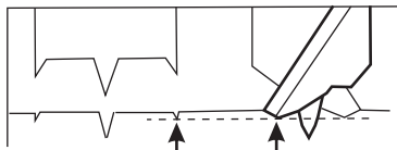
The negative angled tips score the wood before the cutting edges penetrate the wood.
