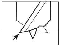
Conventional lip tears wood on entry.
