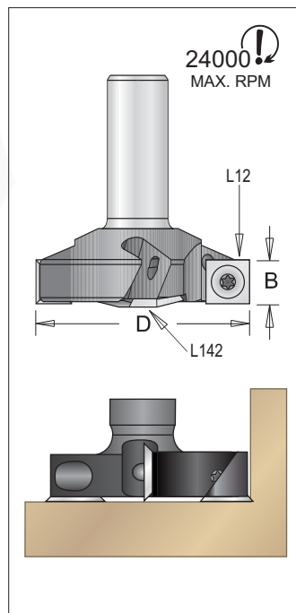
T.C. Knife L12
